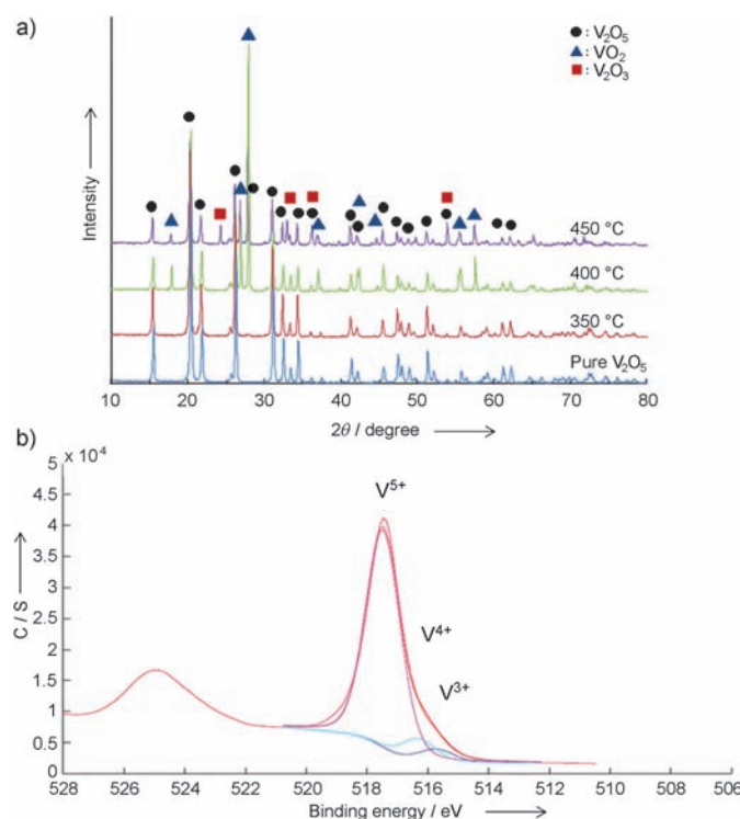
Figure 4. a) XRD patterns of the \text{V}_2\text{O}_5 anode reduced at different temperatures. b) XPS spectrum of the \text{V}_2\text{O}_5 anode reduced at 400 °C.
