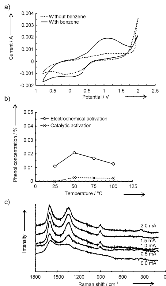
Figure 2. a) I - V profiles of the V 2 O 5 anode with and without the presence of benzene at 50°C. b) Phenol concentration over the V 2 O 5 anode from 25 to 100°C. This plot includes the result for the catalytic reaction between gaseous oxygen and benzene at the open-circuit voltage. c) Raman spectra of the surface of the V 2 O 5 anode at room temperature. Constant currents were applied to the electrochemical cell in ambient atmosphere.
